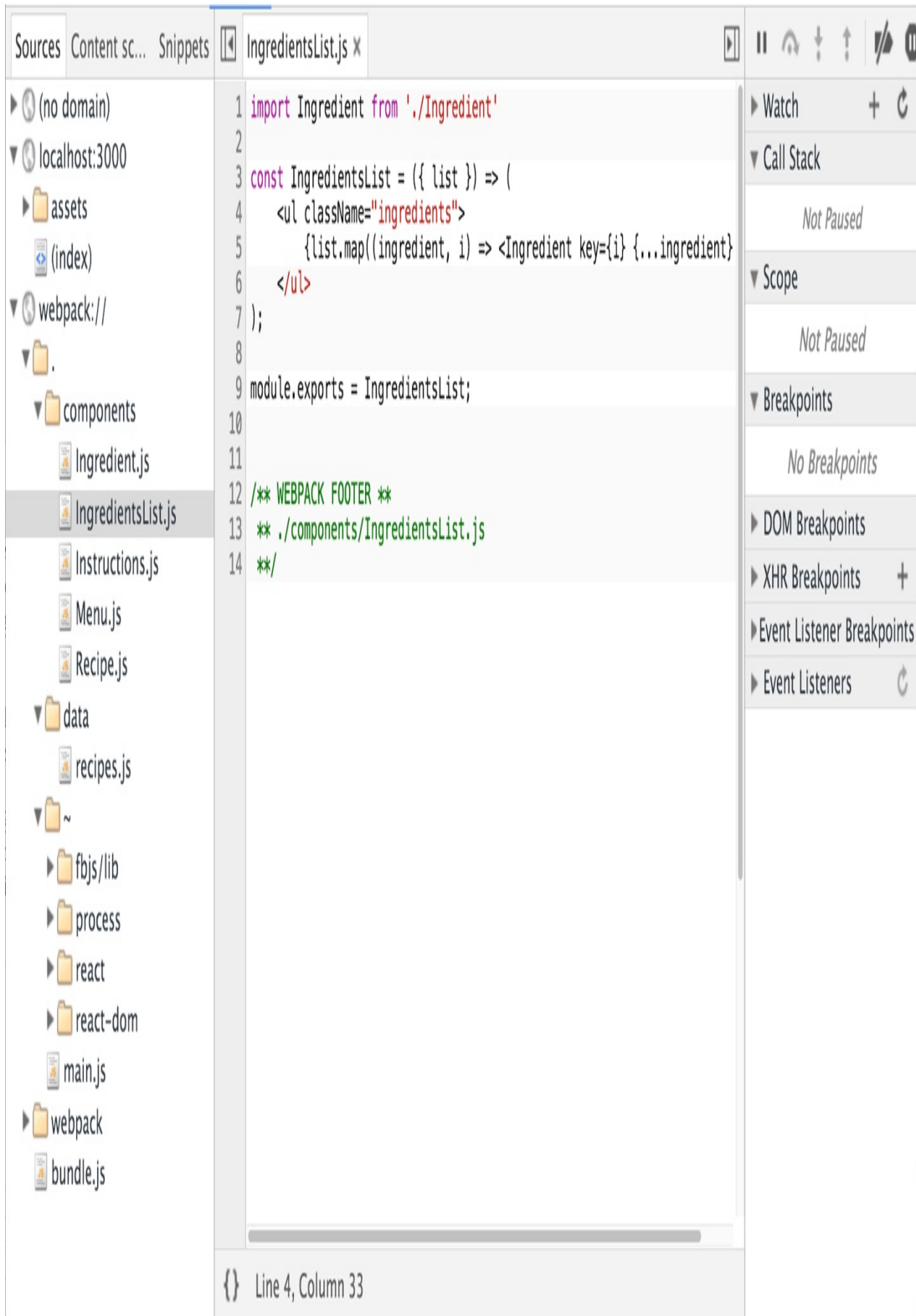
Figure 5-4. Sources panel of Chrome Developer Tools
