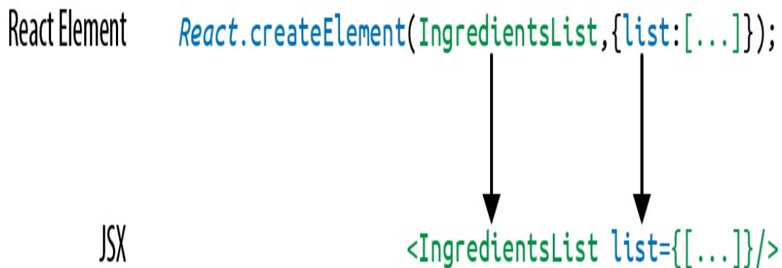
Figure 5-1. Creating the IngredientsList with JSX
