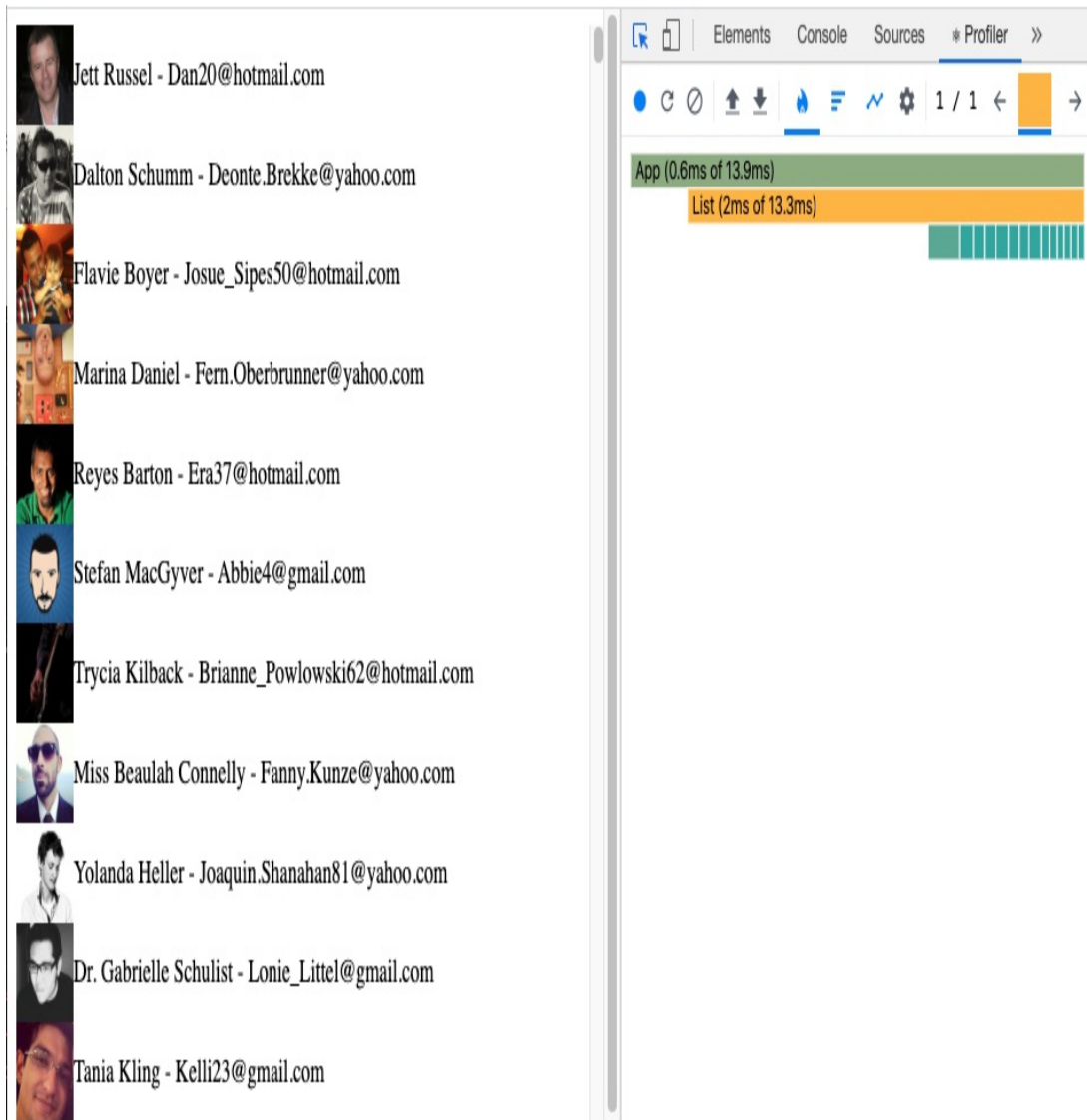
Figure 8-4. 2.6ms for this render
