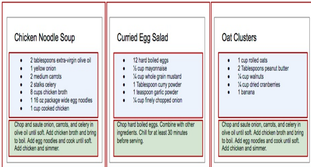
Figure 4-3. Each component is outlined: App , IngredientsList , Instructions
