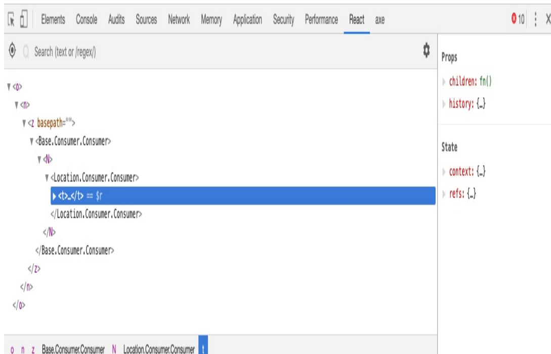
Figure 1-2. Inspecting the DOM with the React Developer Tools
