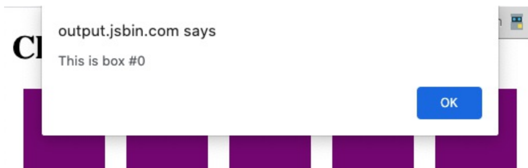
Figure 2-3. The scope of i is protected with let
