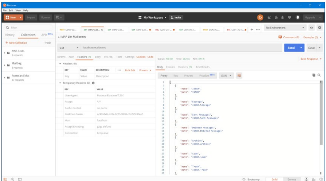
Figure 8-8. An example of using Postman for RESTful web service endpoint function testing
