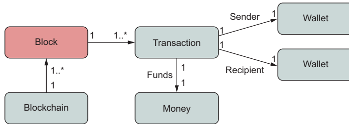
Figure 1.15 The main objects of the domain layer at play in our simple blockchain application
