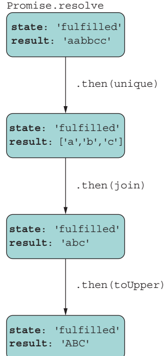
Figure 8.6 Promise chains allow you to manipulate data as a unidirectional, forward conveyor belt where every step applies a different transformation of the data.
