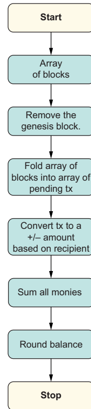
Figure 4.12 Functional flow of control for the logic in calculating a user's total balance in a blockchain
