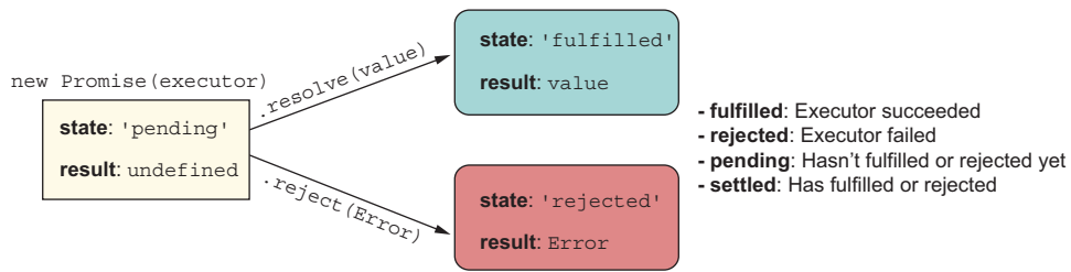
Figure 8.3 The states in which a single Promise object may be its life cycle
