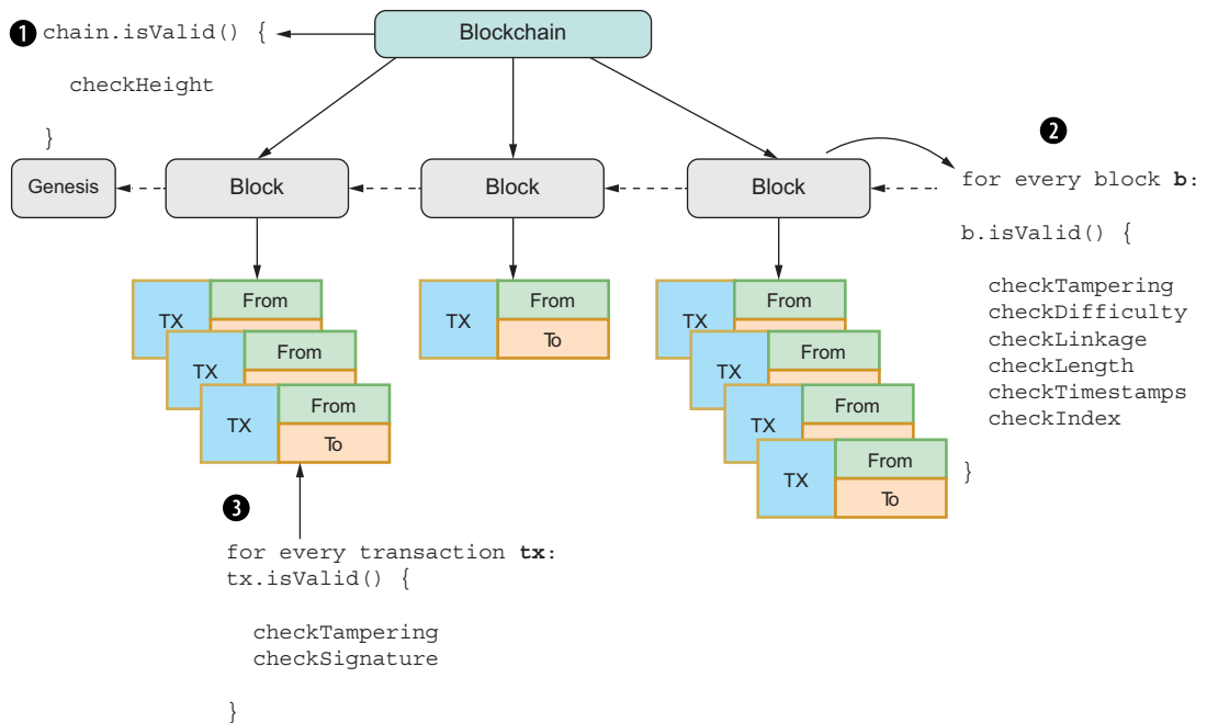
Figure 5.7 Traversing a blockchain's objects, starting with the Blockchain object itself and moving down to each block's transactions. You can think of the routine as forming a treelike structure, with the Blockchain object itself as the root, blocks as the second-level nodes, and transactions as the leaves of the tree.
