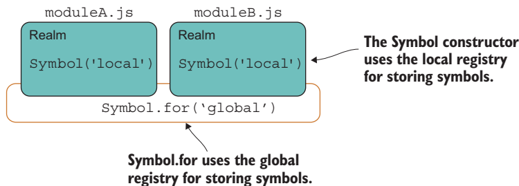
Figure 7.1 Scope of the local and global registries
