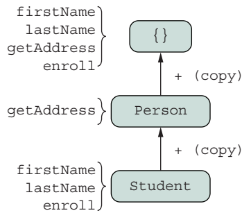
Figure 1.2 Two concrete objects (Student and Person) mesh into a brand new object with all properties assigned from the combined objects. Although no prototypical inheritance is at play here, the directions of the arrow is kept the same as in figure 1.1 to convey the similar mental model of both approaches.
