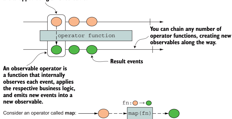
Figure 1.12 A source Observable object (first long arrow) with all its events piped into an operator function and transformed. All new values are emitted by means of a new Observable .
