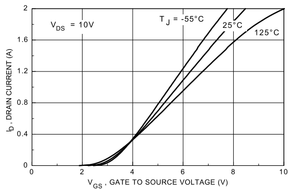
Figure 5. Transfer Characteristics
