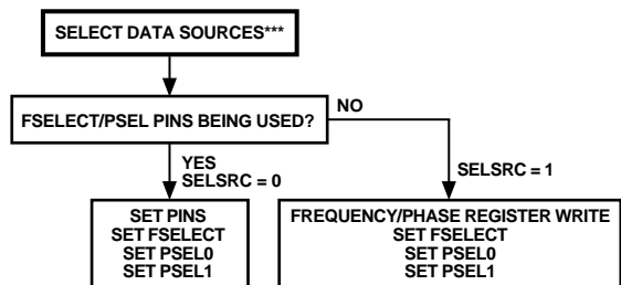
Figure 23. Selecting Data Sources
