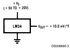
FIGURE 1. Basic Fahrenheit Temperature Sensor (+5° to +300°F)
