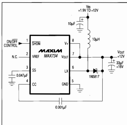
Figure 3. Bootstrap Operation
