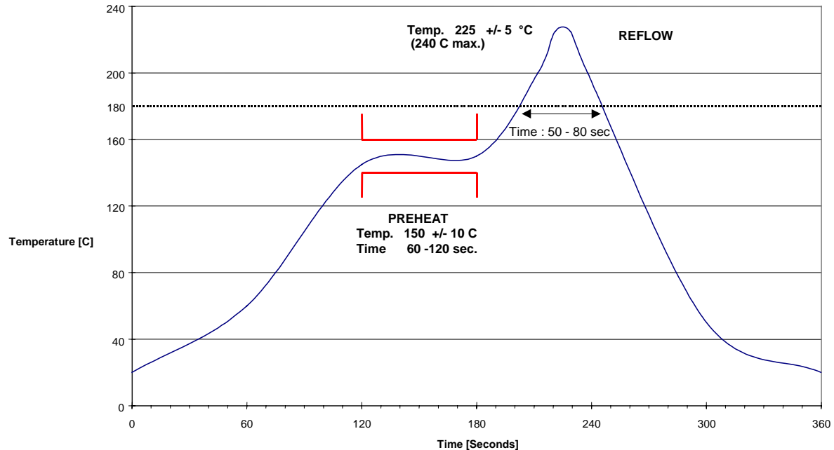
Figure 11: Recommended soldering profile
