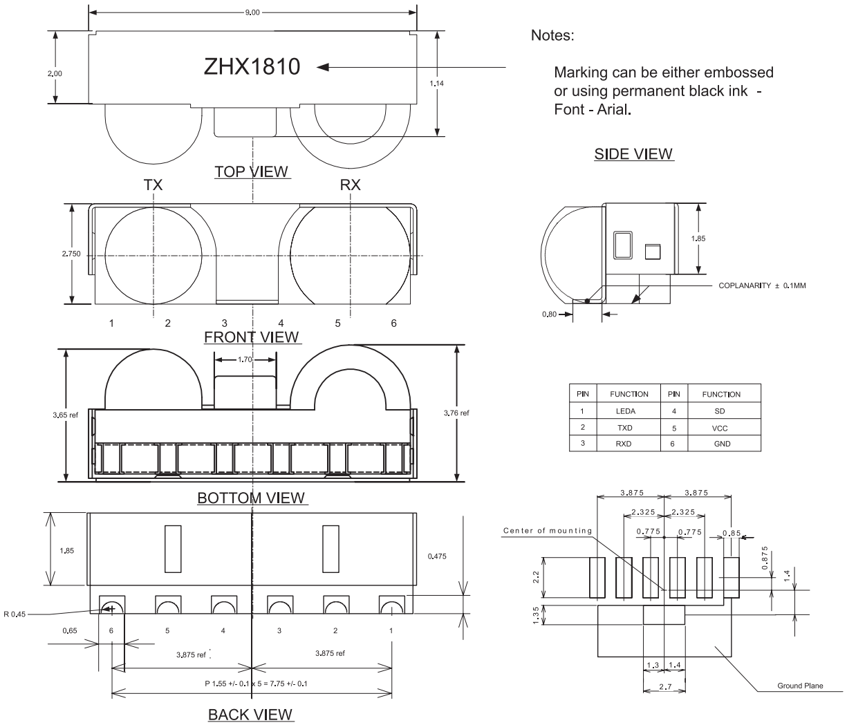
Figure 8. Alternative ZHX1810 Mechanical Drawing
