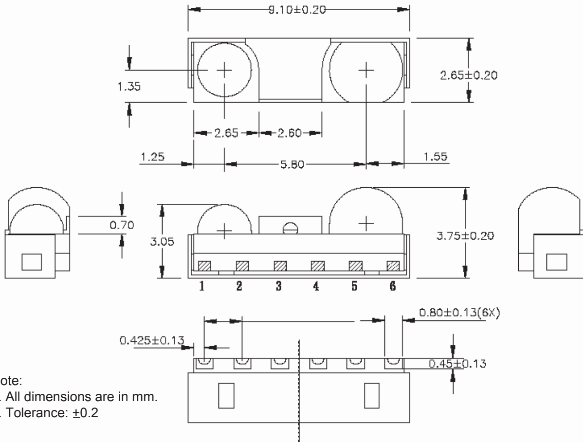
Figure 9. Alternative ZHX1810 Mechanical Drawing
