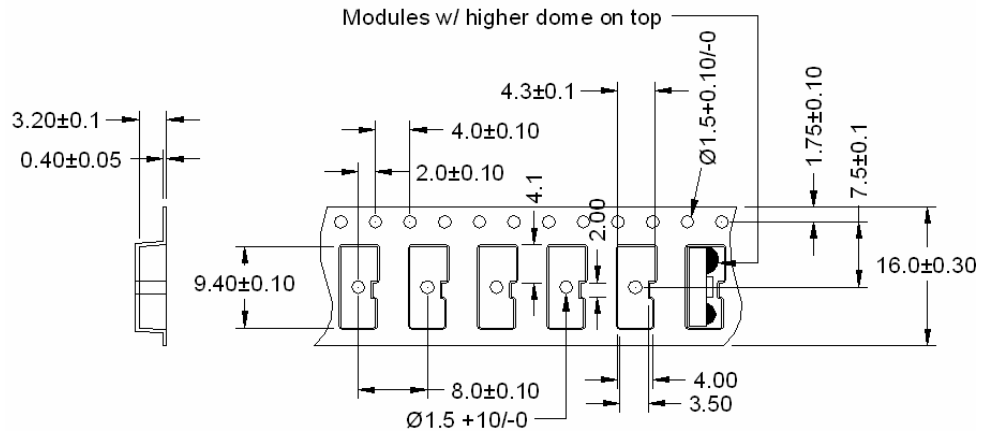
Figure 14. Alternative ZHX1810 Tape Dimensions and Configuration (Unit: mm)
