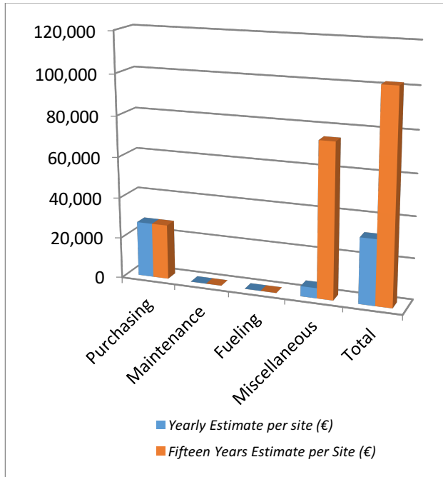
Fig.5, Estimated cost for solar photovoltaic power system base station per site.
