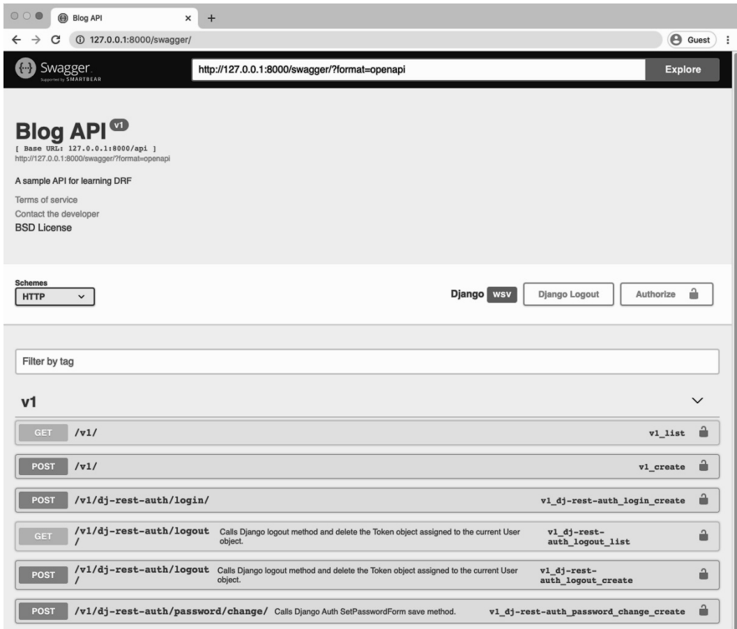
Swagger view
