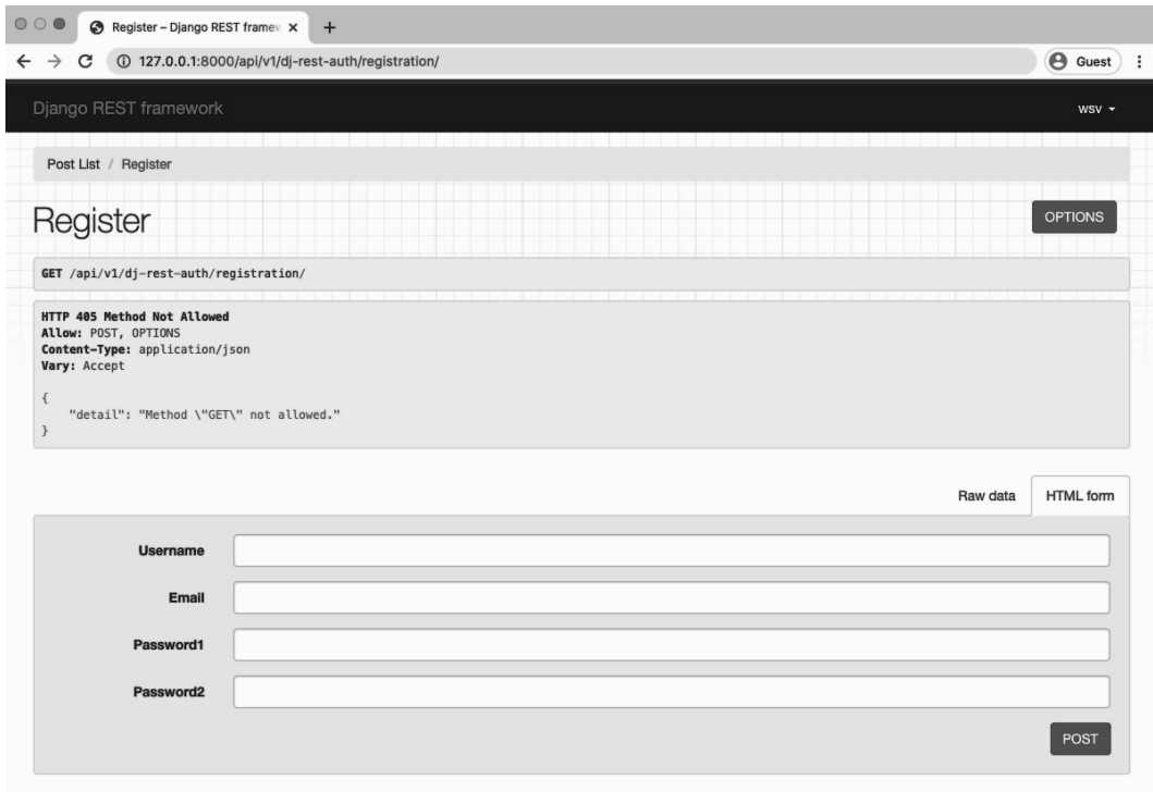
API Register
