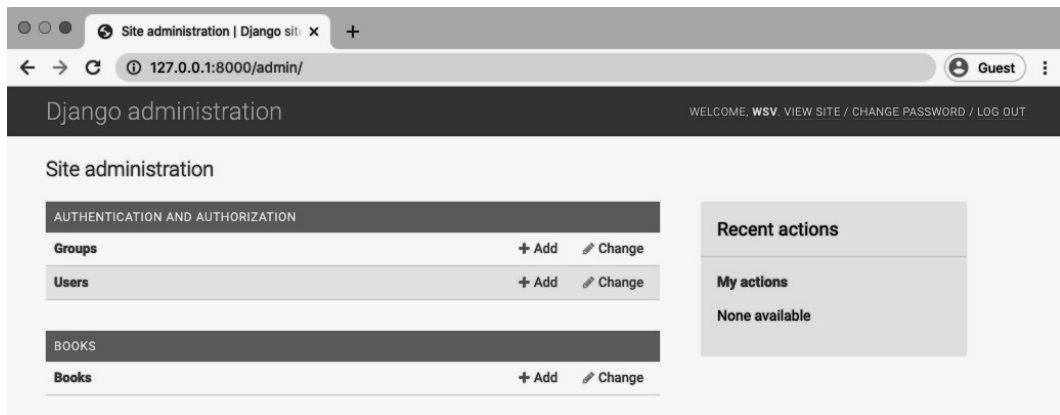
Admin homepage
