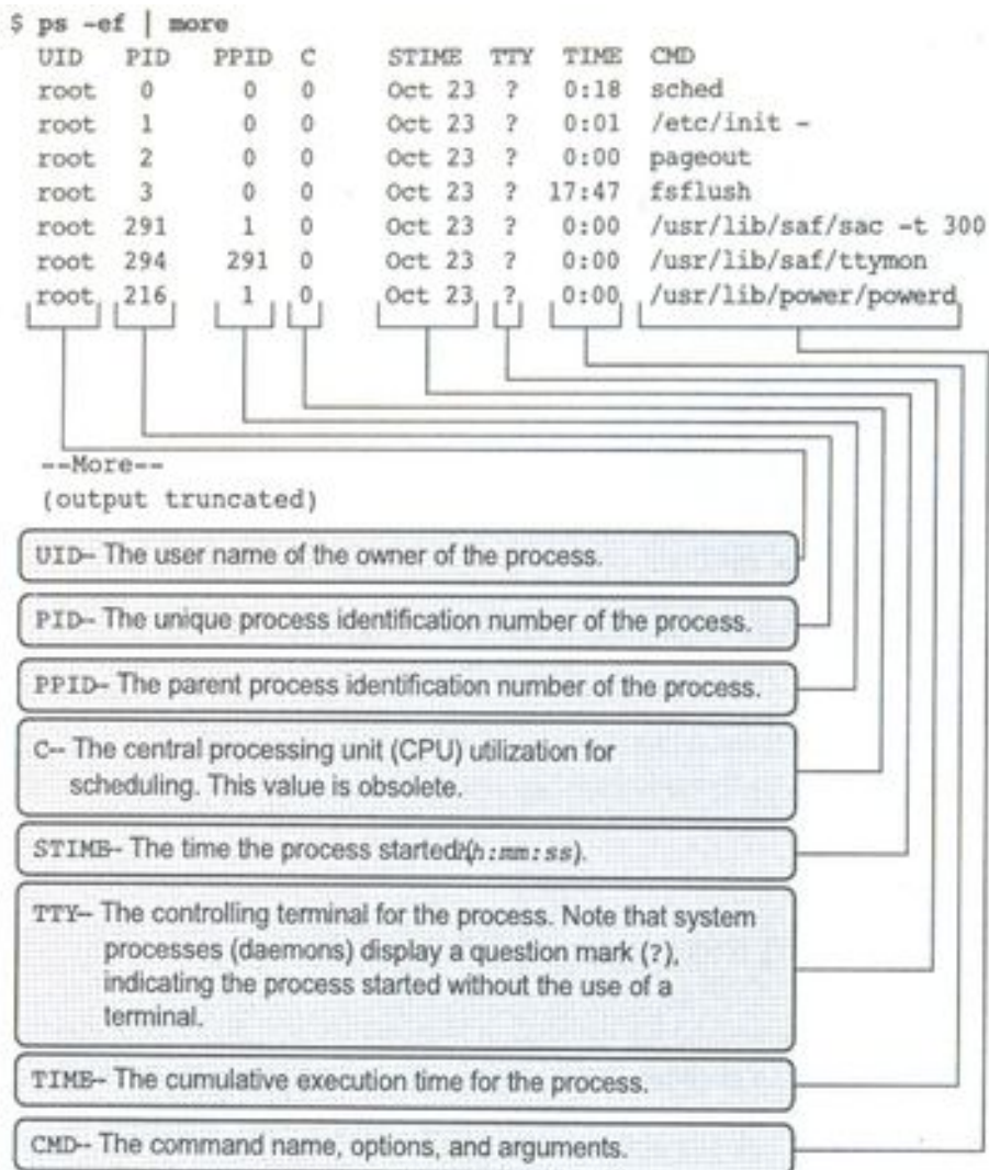
The ps -ef Command Output Description
